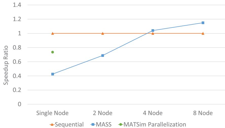
Figure 8: Execution comparison with sequential version
