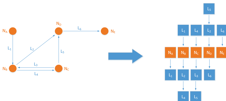
Figure 4: Network mapping using adjacent list
