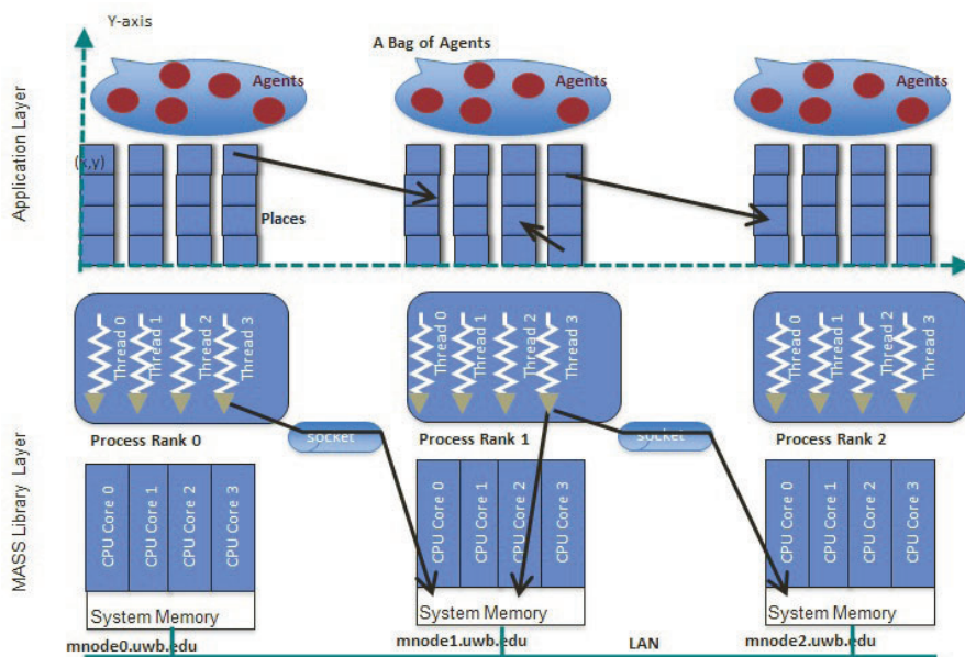
Figure 1: The MASS library's execution model
