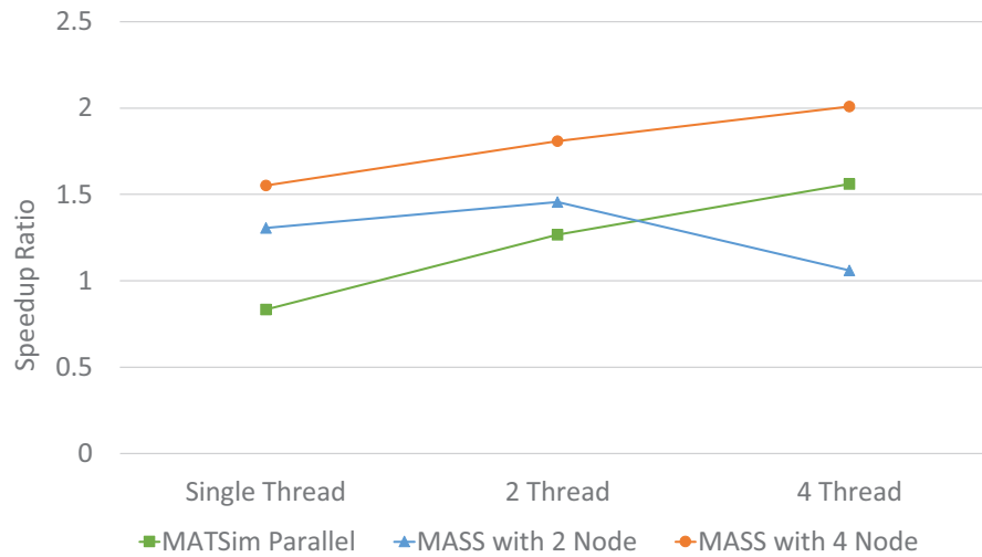
Figure 9: Execution comparison with parallelized MATSim
