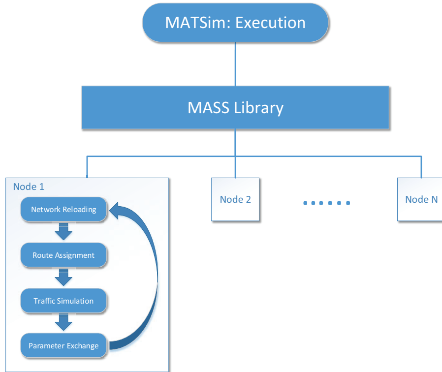
Figure 3: MASS-parallelized MATSim's system overview
